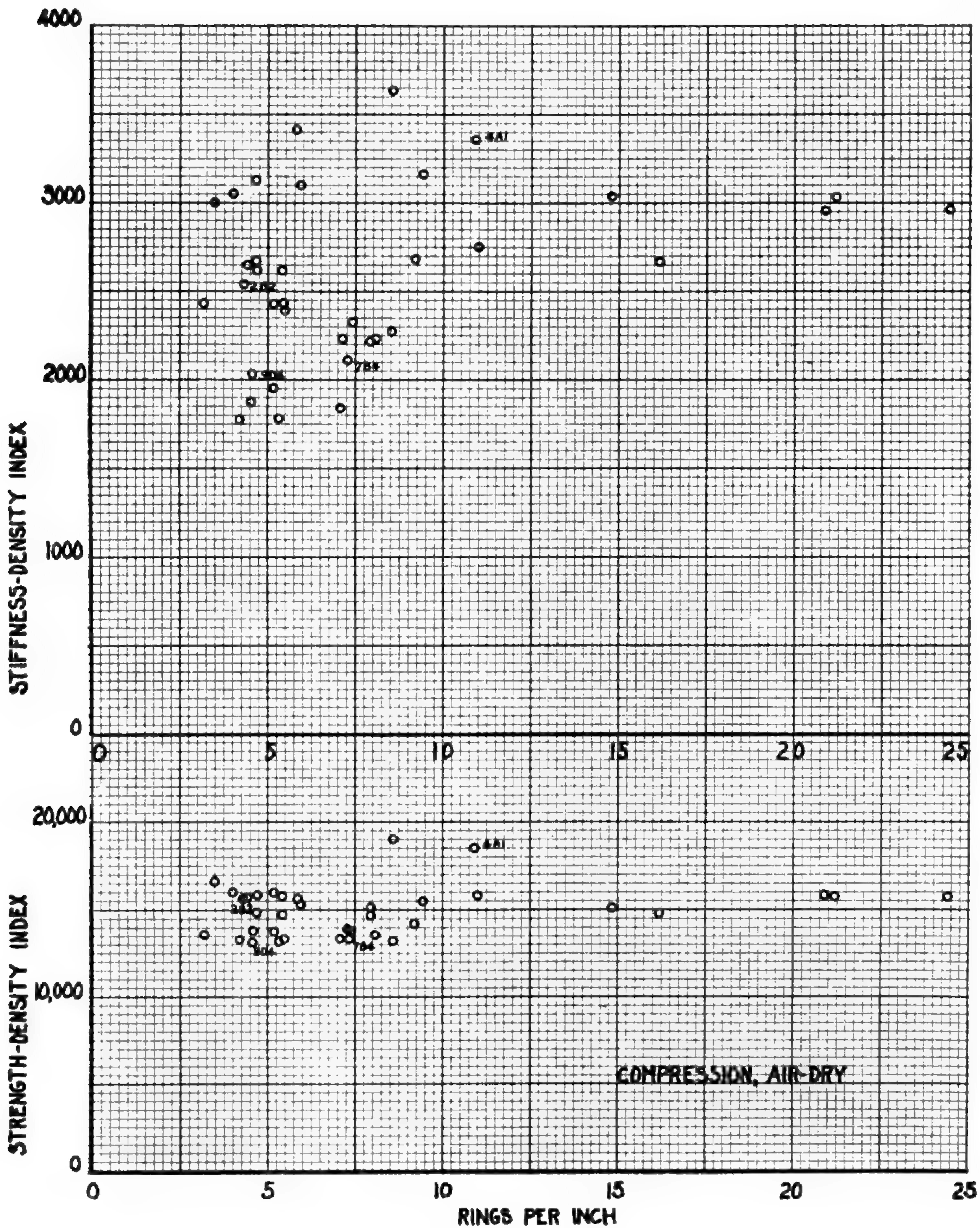
Fig. 9. Axial compression strength-density index (ultimate strength \div specific gravity) and stiffness-density index (modulus of elasticity \div specific gravity) plotted over growth rate for air-dry specimens.
